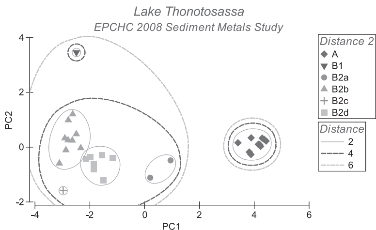
FIG. 3. PCA plot of Lake Thonotosassa sediment metals with Euclidian distance groups.
