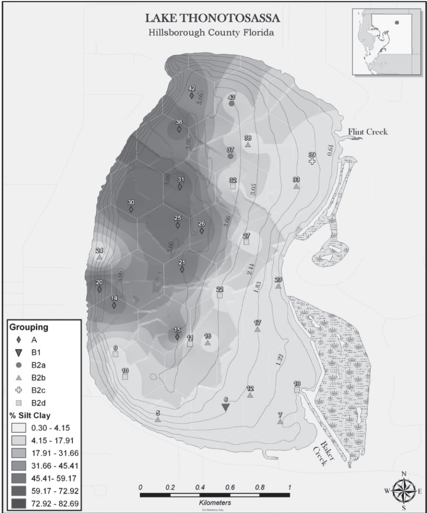
FIG. 1. EPCHC Lake Thonotosassa sediment sampling grid (hexagons) and sample locations, May 2008. Lake bathymetry indicated in 0.61 meter (2 feet) intervals [modified from Kenner (1964) and Harley and Eilers (2008)]. Shading represents % silt + clay distribution. Symbols represent cluster groupings from the Euclidian distance cluster analysis (see Figure 2).
