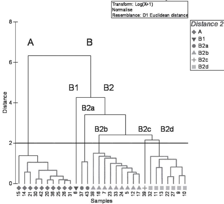
FIG. 2. Euclidian distance cluster analysis of Lake Thonotosassa sediment metals (excluding Al and Fe). Data log (n+1) transformed and normalized for analysis.
