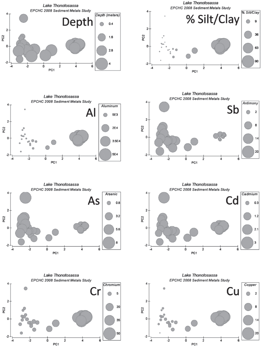
FIG. 4. PCA bubble plots for depth (m), silt + clay (%), and individual metals (mg/kg).
